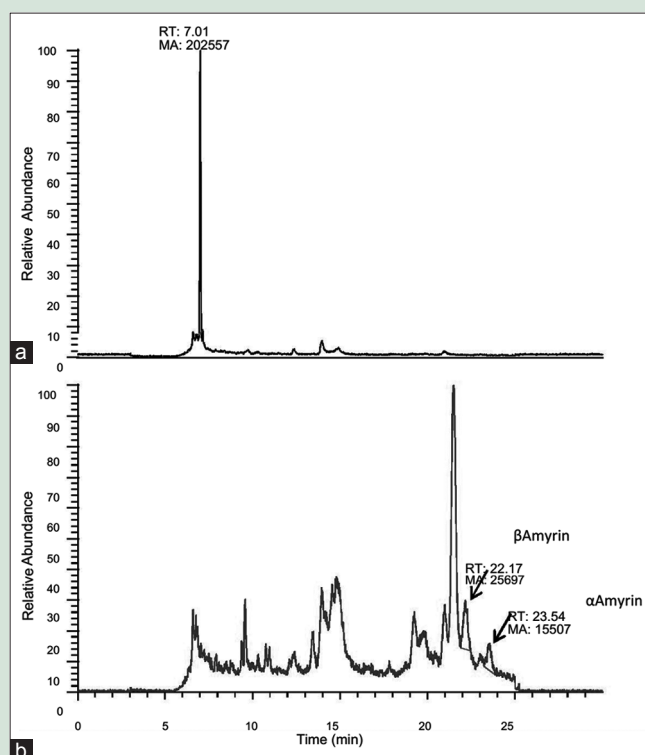
Figure 1: High-performance liquid chromatography chromatogram of (a) estrone (Internal standard for analysis of terpenes) (b) Costus pictus extract
