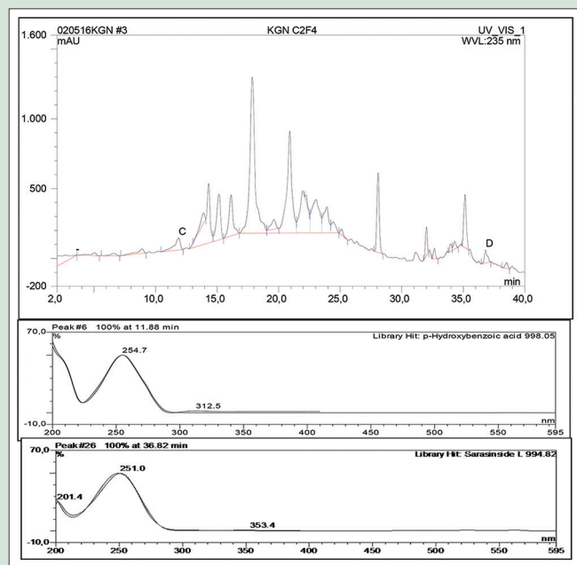
Figure 2: High-pressure liquid chromatography chromatogram of n-hexane fraction (AC2) and UV chromatogram of p-Hydroxybenzoic acid and UV chromatogram of Sarasinside L. C: p-Hydroxybenzoic acid; D: Sarasinside L
