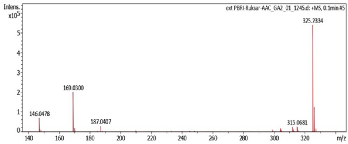
Figure 3: Mass spectra of the isolated compound (Fraction A) of AA.
